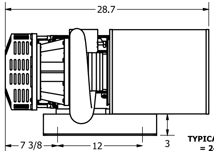
8008256 FILTER / SILENCER
